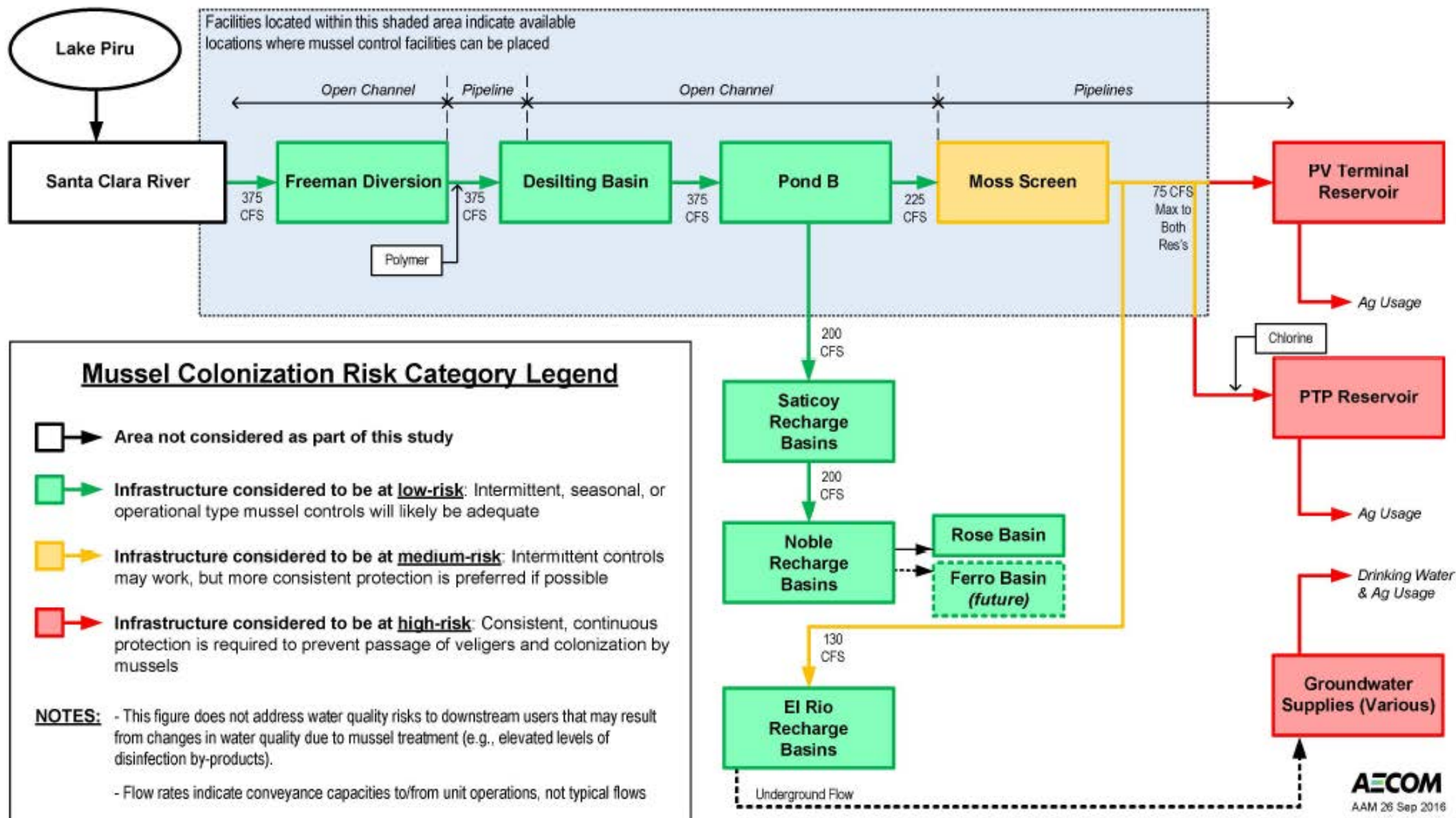
Figure 6-1. Infrastructure Overview and Locations Requiring Veliger/Mussel Control
